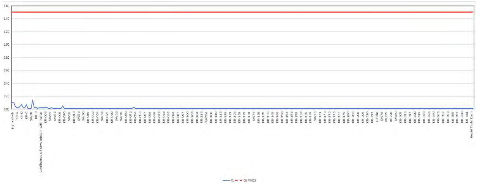
Figure 4-63: Concentration of copper in Kafue River
