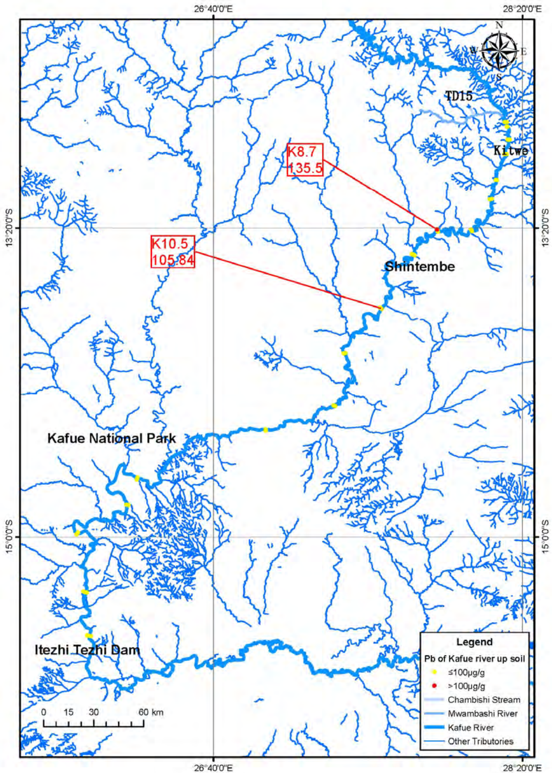
Figure 6-21: Distribution of Lead in Kafue River
