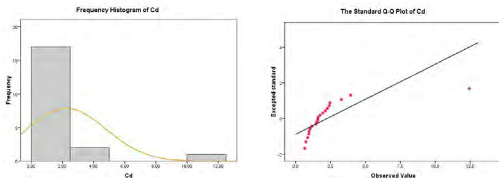
Figure 6-25: Frequency histogram and Q-Q diagram of Cd
