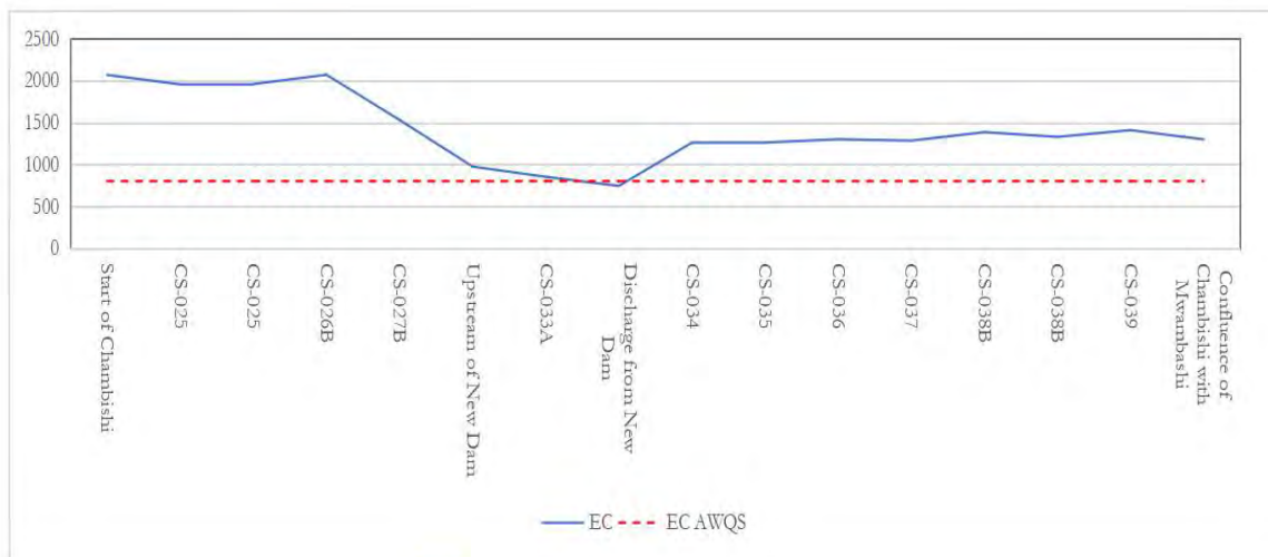
Figure 4-45: Electrical conductivity along Chambishi Stream
