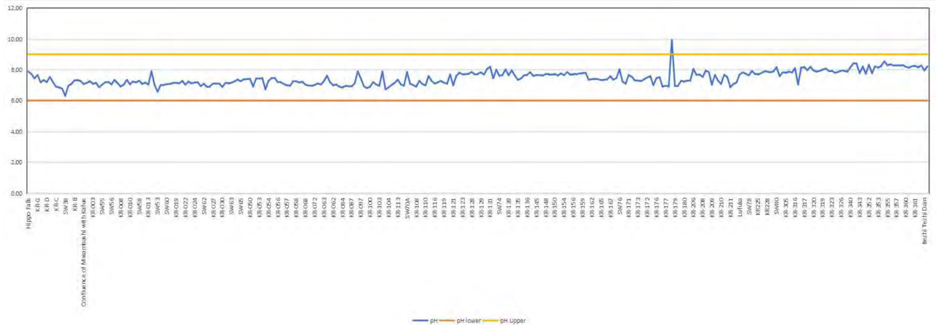
Figure 4-62: pH of water along Kafue River
