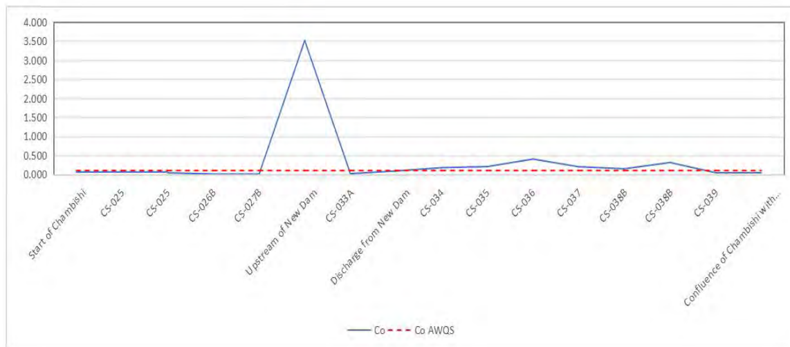
Figure 4-48: Concentration of cobalt in Chambishi Stream
