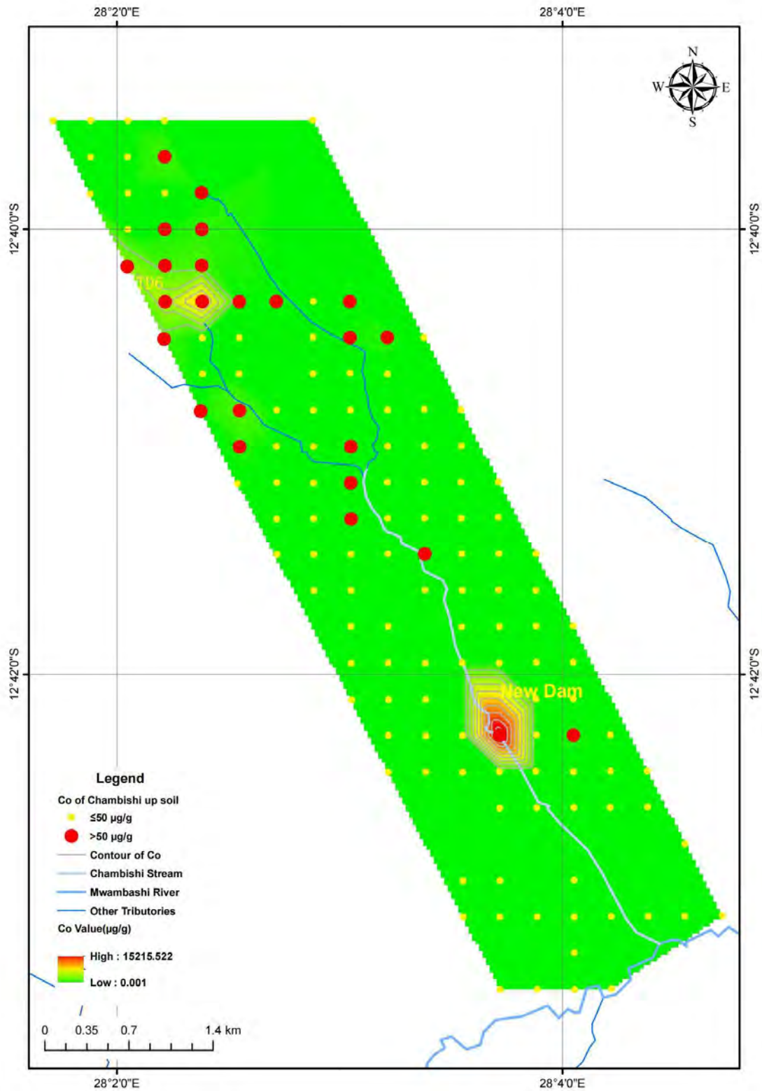
Figure 6-41: Distribution of Co Exceeding Baseline Value
