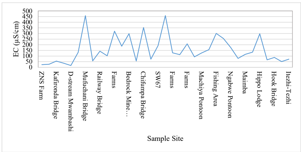
Figure 4-38: Graph showing EC in sediment
