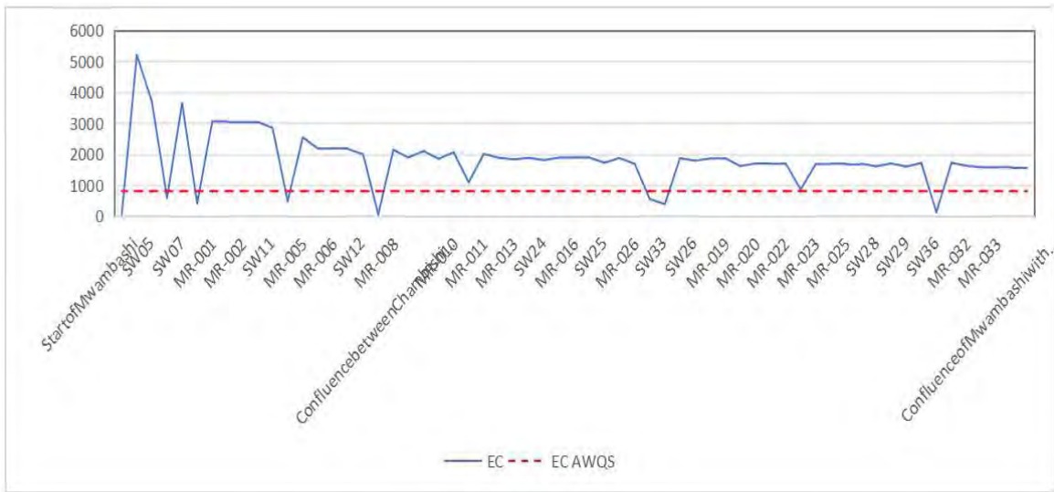
Figure 4-53: Electrical conductivity along Mwambashi River
