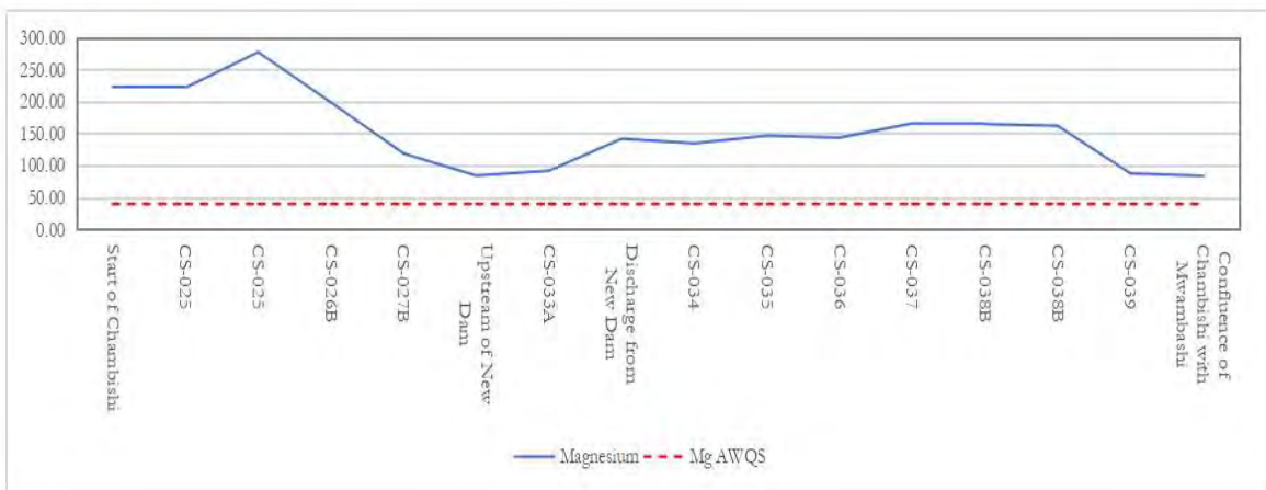
Figure 4-51: Concentration of magnesium in Chambishi Stream
