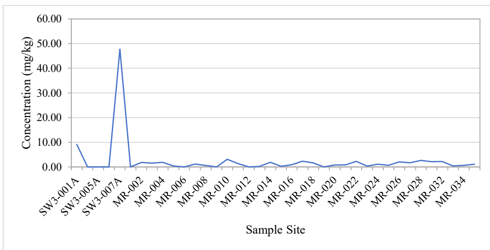
Figure 4-33: Graph showing the concentration of arsenic in sediment
