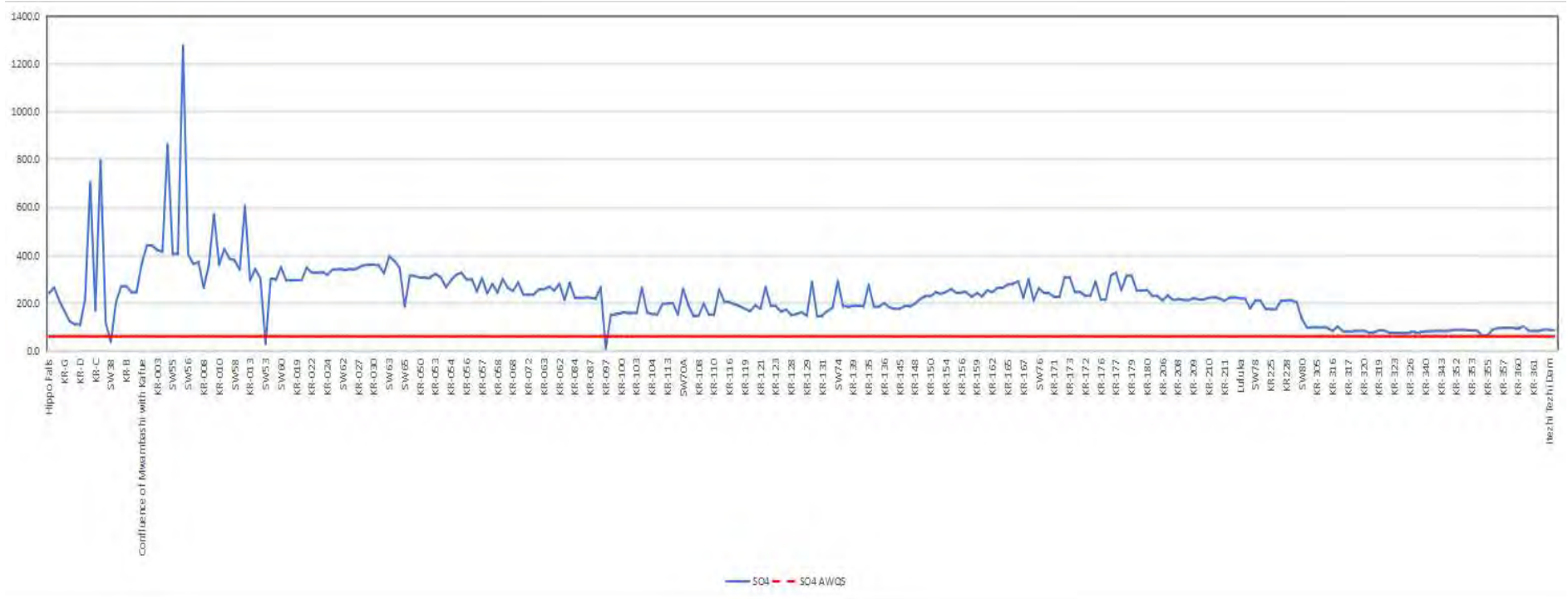
Figure 4-66: Concentration of sulphates in Kafue River
