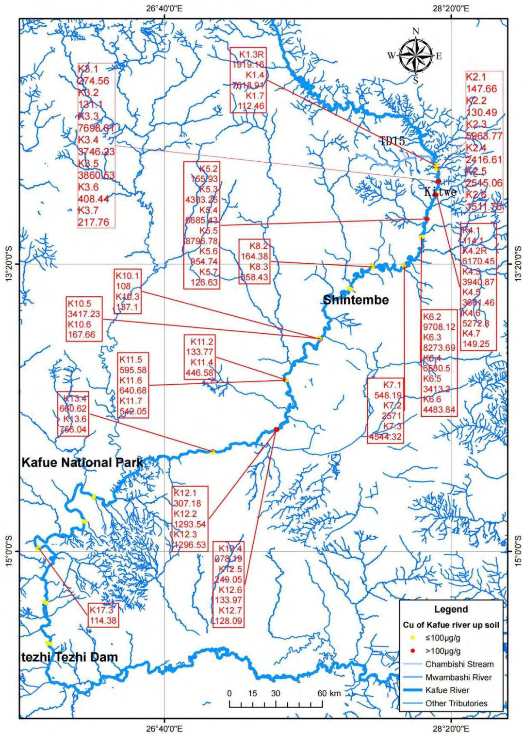
Figure 6-20: Distribution of Copper in Kafue River
