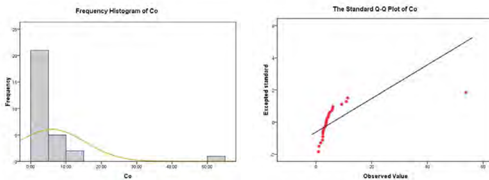
Figure 6-36: Frequency histogram and Q-Q diagram of Co
