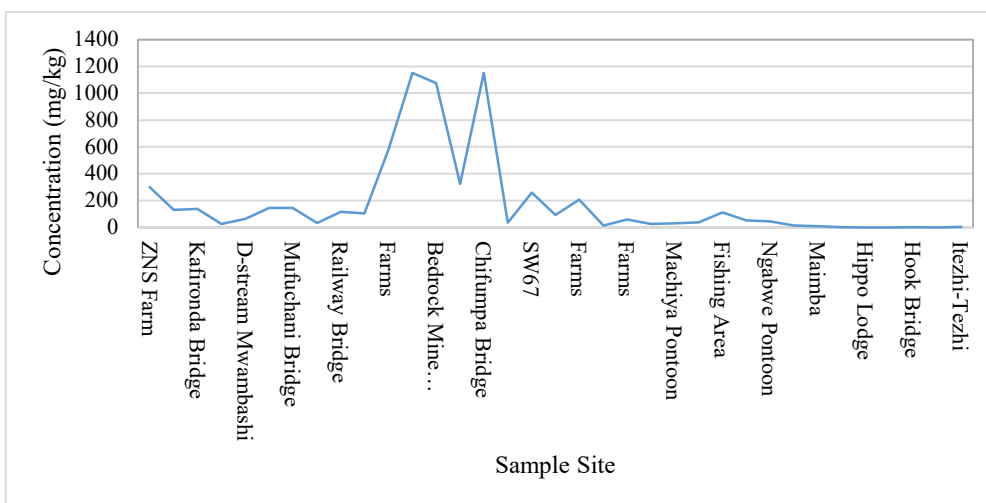
Figure 4-40 showing the concentration of Cobalt in sediment
