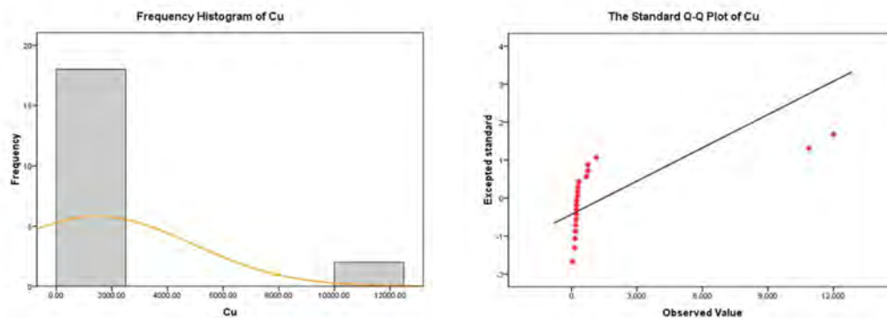
Figure 6-27: Frequency histogram and Q-Q diagram of Cu
