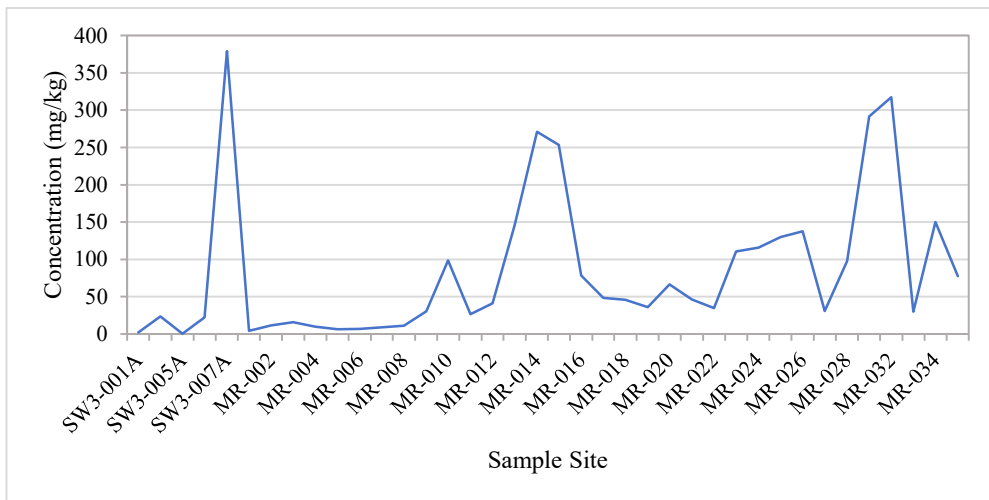
Figure 4-32 showing the concentration of Cobalt in sediment
