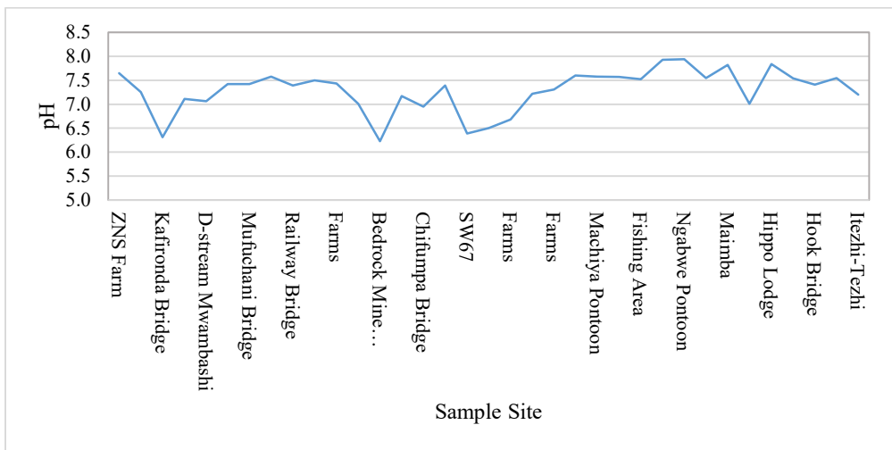
Figure 4-37: Graph showing the pH in sediment
