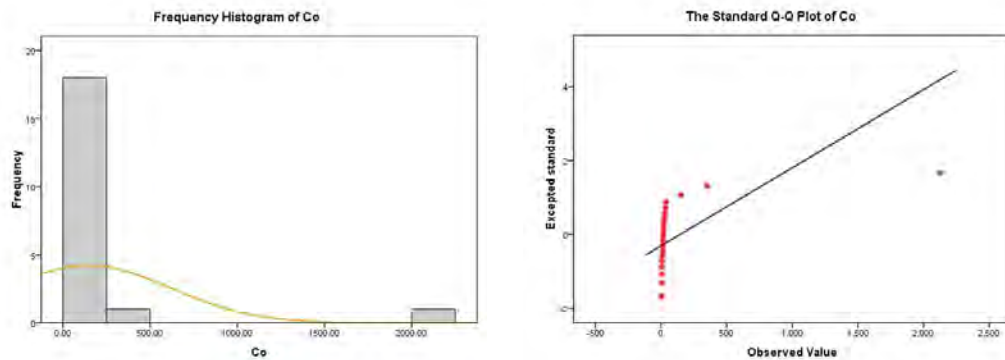
Figure 6-26: Frequency histogram and Q-Q diagram of Co
