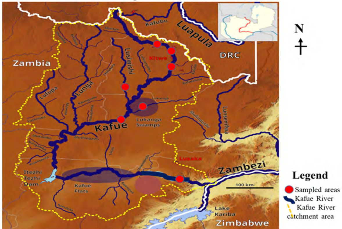
Figure 11-1: Map showing sampling localities across the Kafue River system
