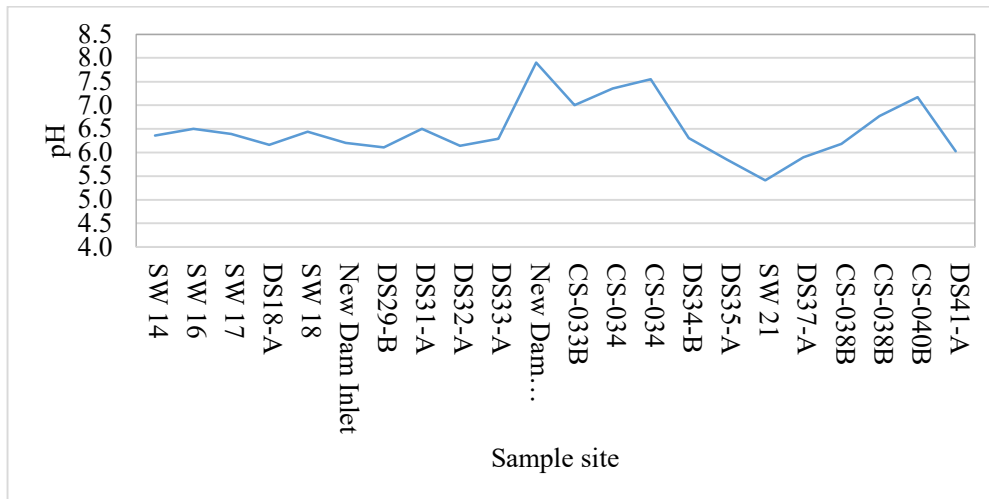
Figure 4-21: Graph showing the pH in sediment
