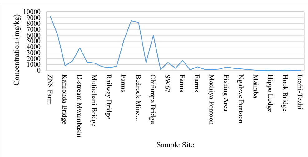
Figure 4-39: Graph showing the concentration of copper in sedimentt
