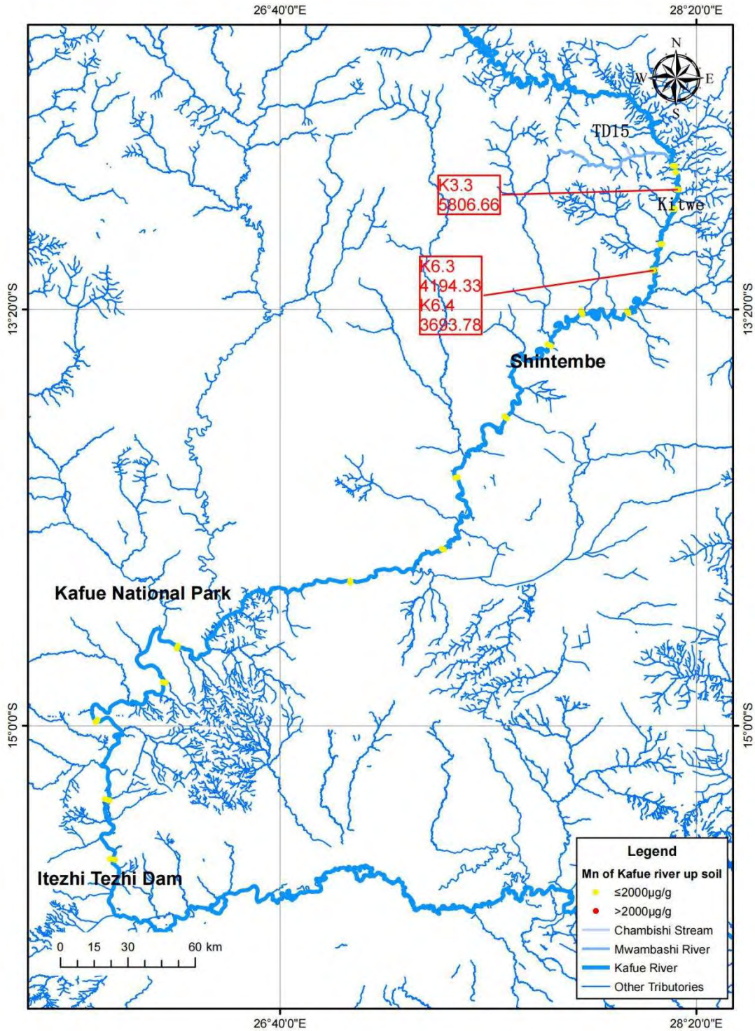
Figure 6-22: Distribution of Manganese in Kafue River
