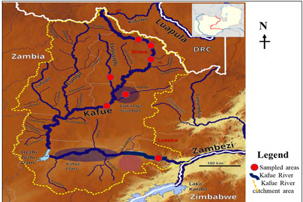
Figure 11-4: Map showing sampling localities across the Kafue River system
