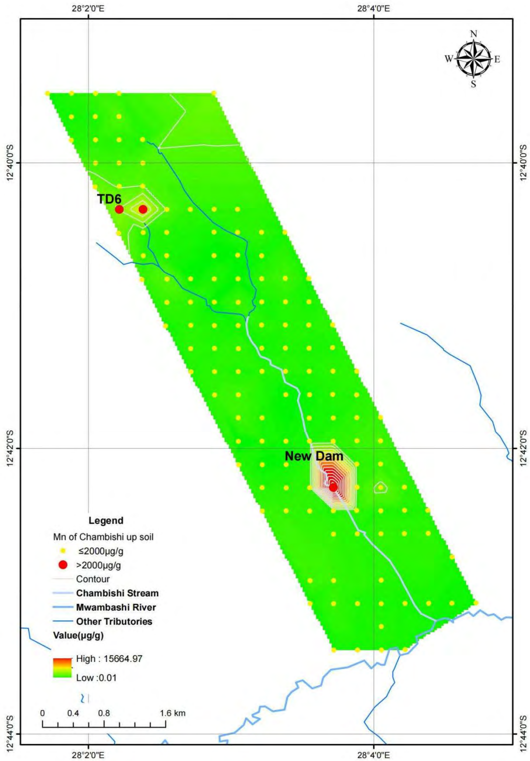
Figure 6-14: Distribution of Manganese in Chambishi Stream
