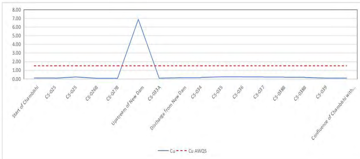
Figure 4-47: Concentration of copper in Chambishi Stream
