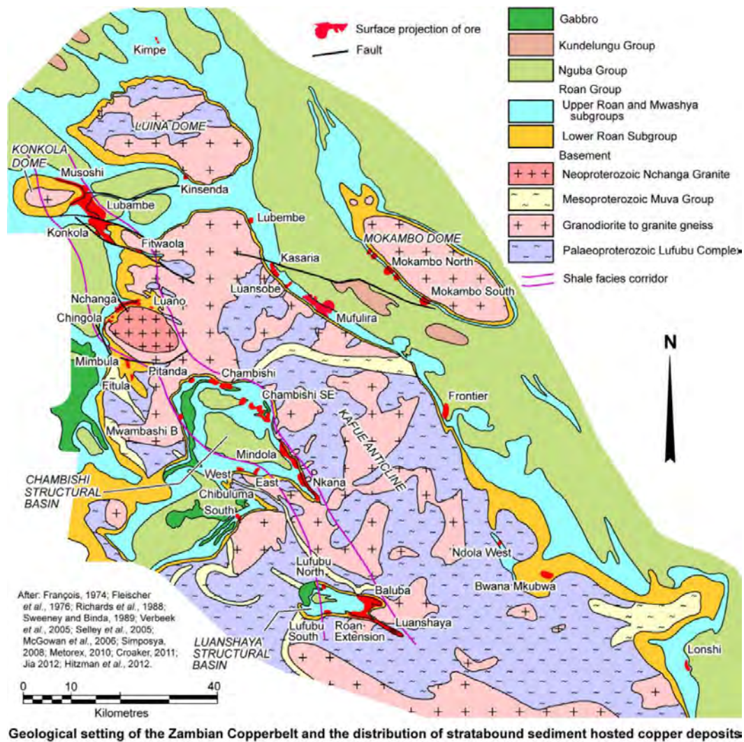
Figure 5-8: Geological setting of the Zambia Copperbelt 10
