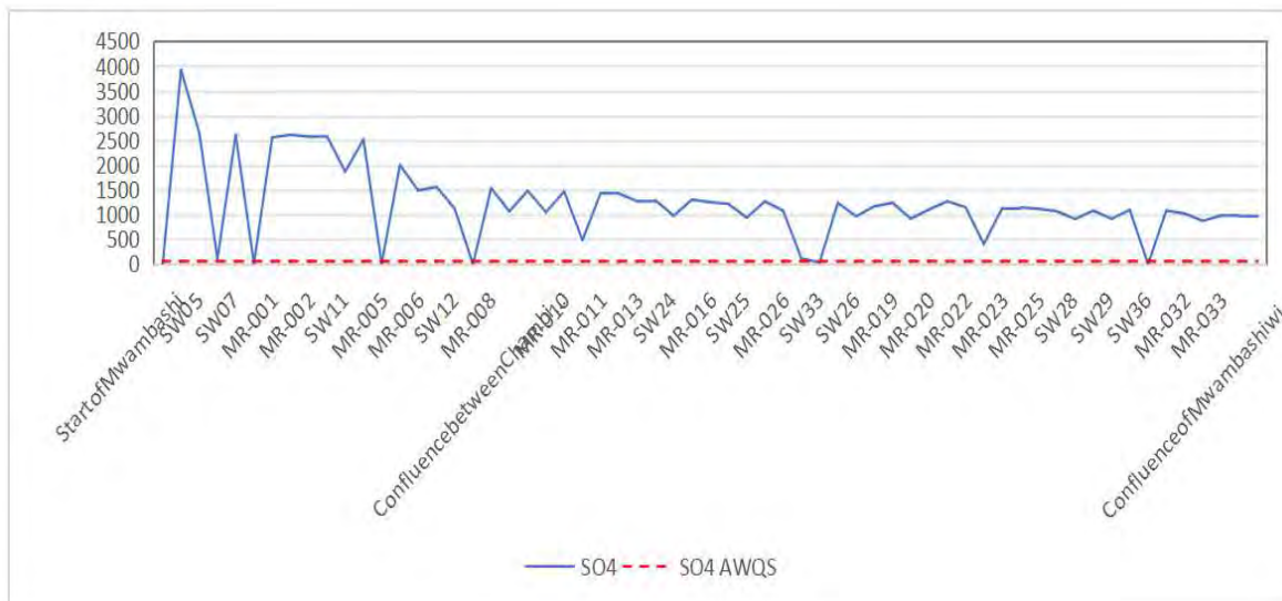
Figure 4-58: Concentration of sulphates in Mwambashi River
