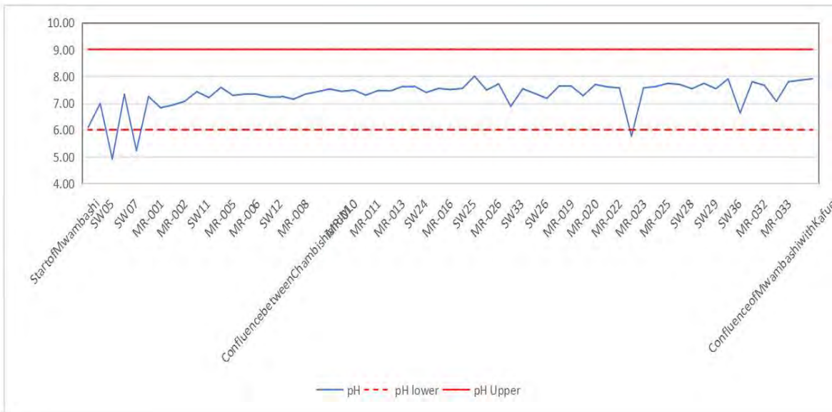
Figure 4-54: pH of water along Mwambashi River
