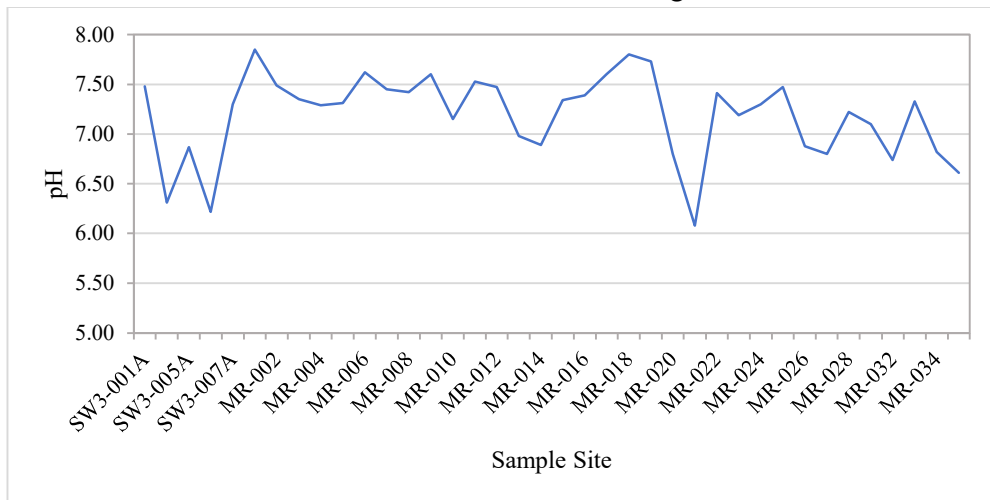
Figure 4-29: Graph showing the pH in sediment
