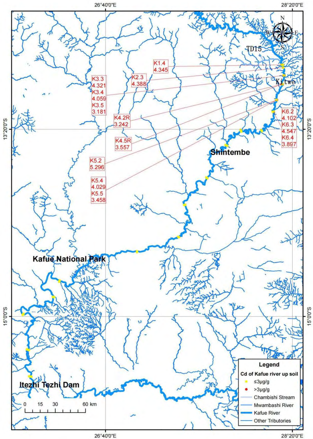
Figure 6-24: Distribution of Cadmium in Kafue River
