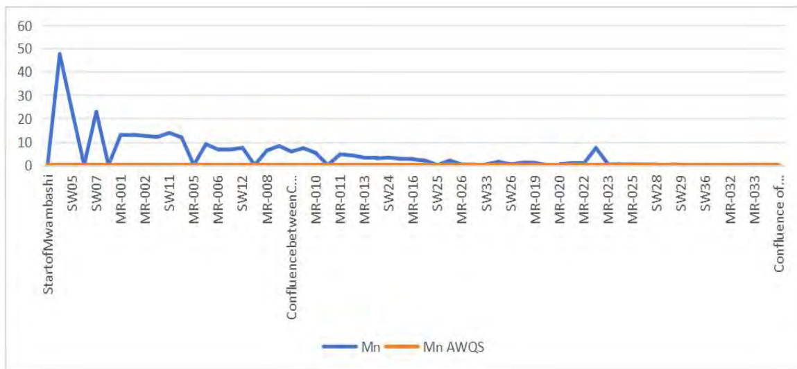
Figure 4-57: Concentration of Manganese in Mwambashi River
