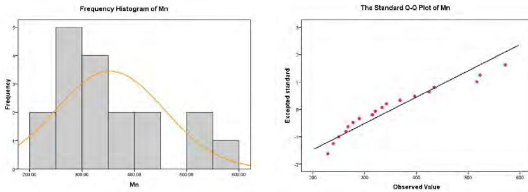
Figure 6-35: Frequency histogram and Q-Q diagram of Mn
