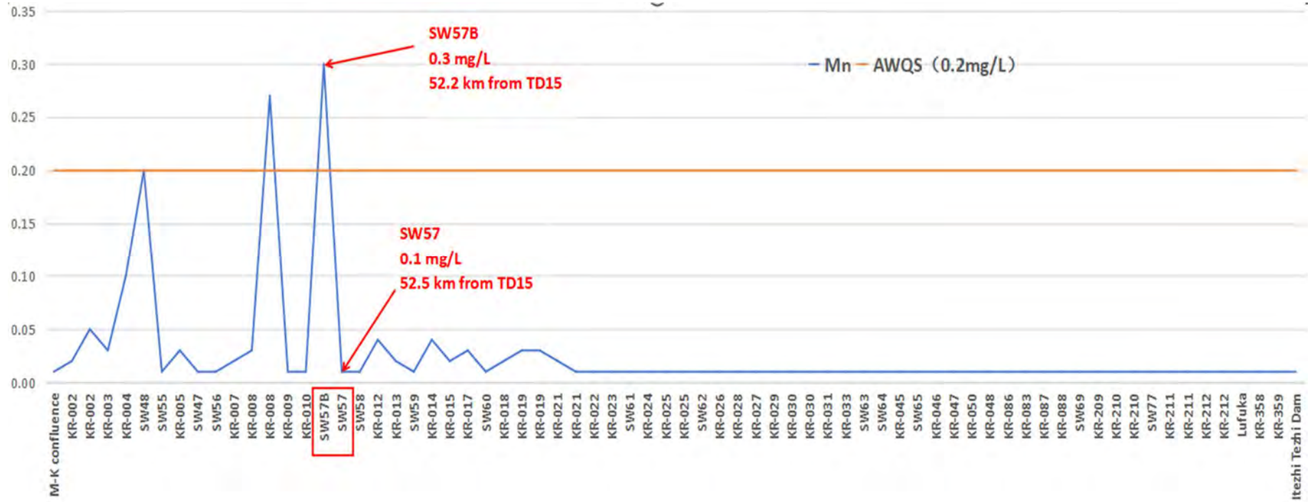
Figure 4-69: Distribution of Manganese Concentration along Kafue River
