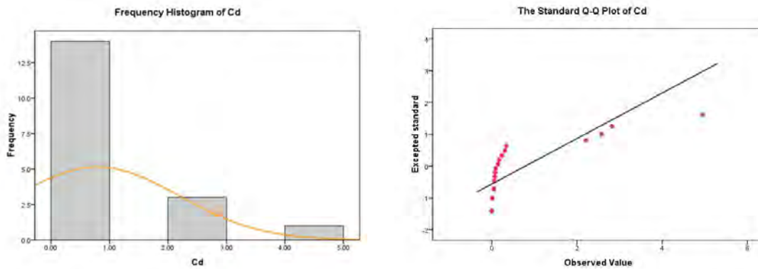
Figure 6-29: Frequency histogram and Q-Q diagram of Cd
