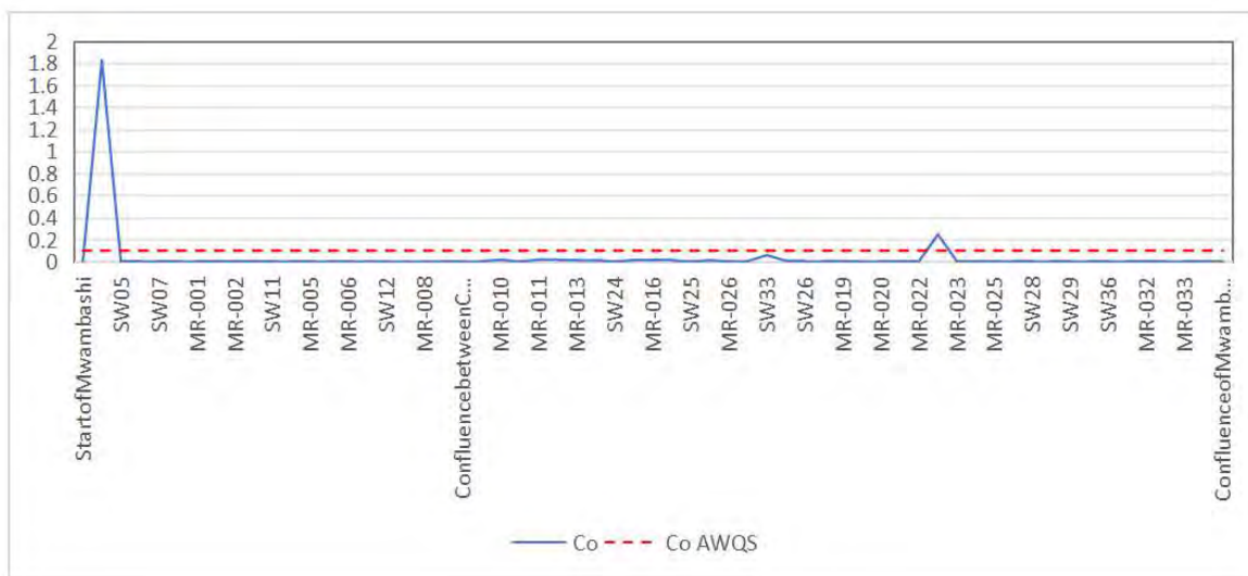
Figure 4-56: Concentration of Cobalt in Mwambashi River
