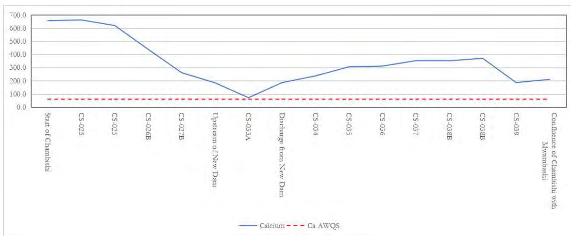
Figure 4-52: Concentration of calcium in Chambishi Stream
