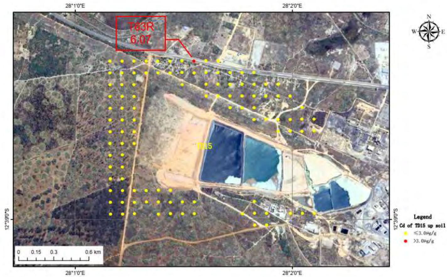
Figure 6–8: Distribution of Cadmium in TD 15
