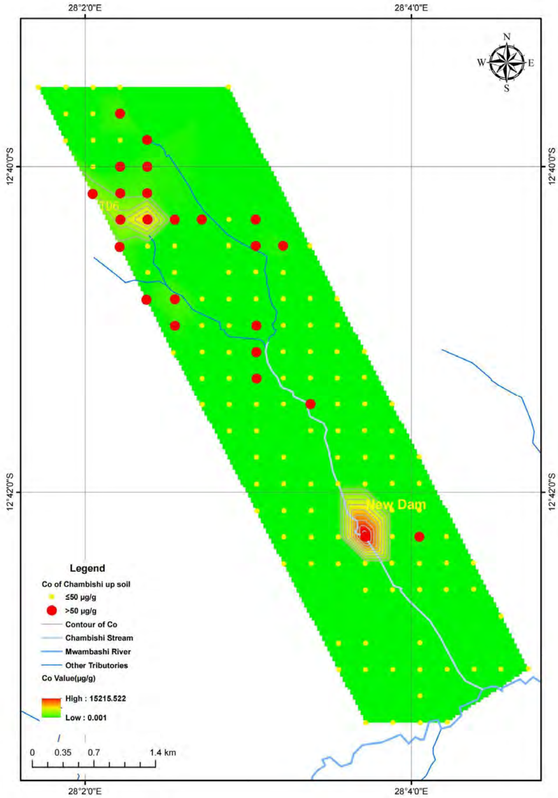
Figure 6-12: Distribution of Cobalt in Chambishi Stream
