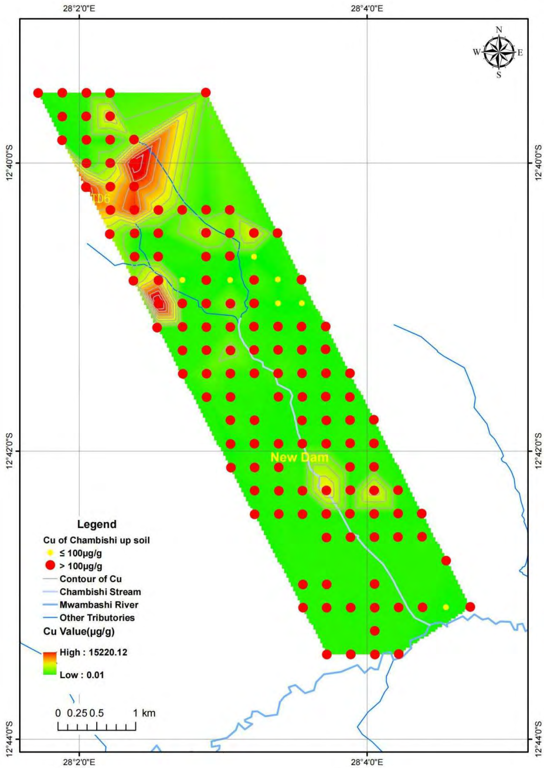
Figure 6-13: Distribution of Copper in Chambishi Stream
