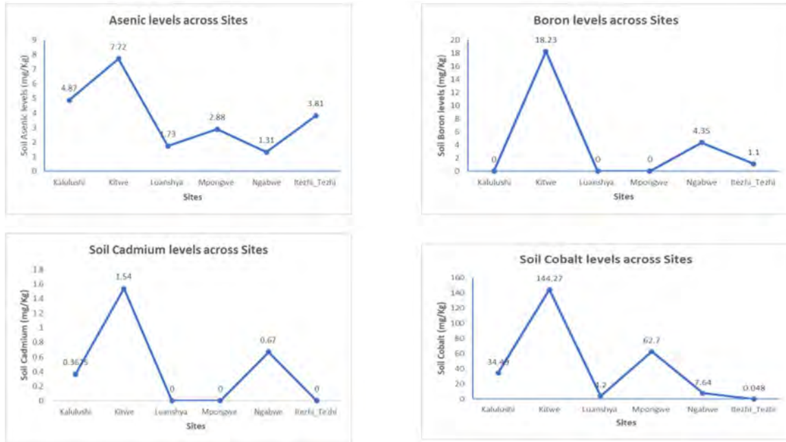
Figure 8 - 1: Selected soil chemical elements across the different sites
