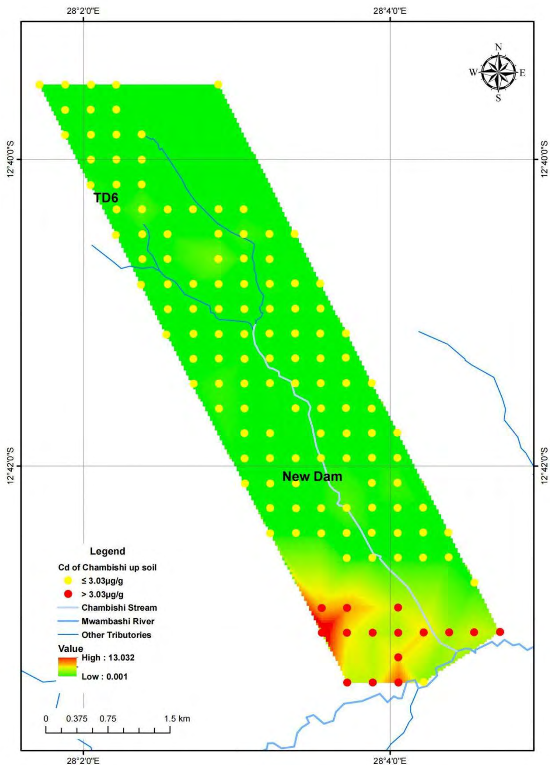
Figure 6-40: Distribution of Cd Exceeding Baseline Value
