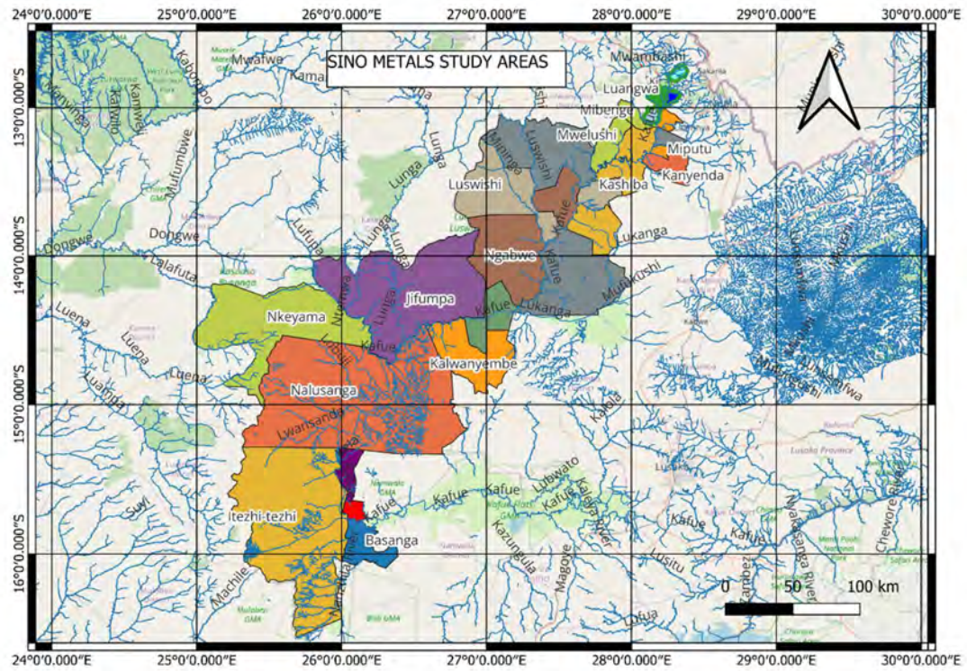
Figure 7-17: Anthropogenic Zones
