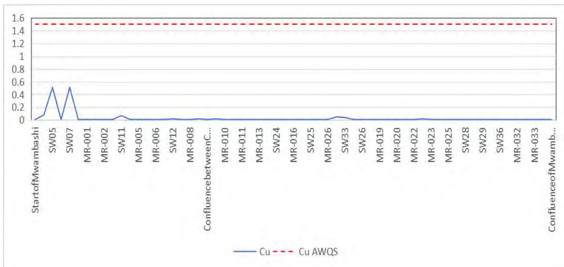
Figure 4-55: Concentration of Copper in Mwambashi River
