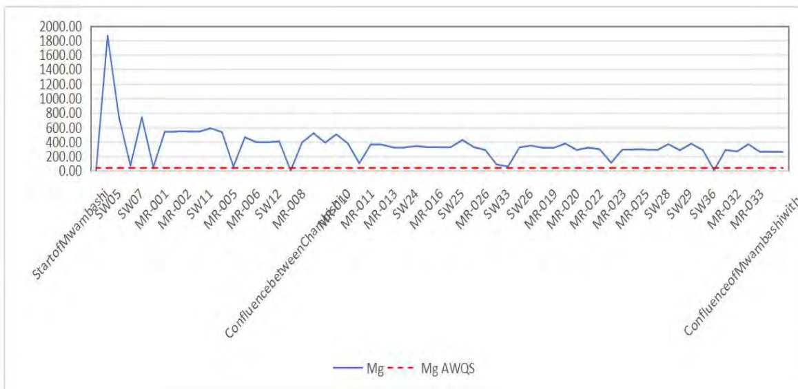
Figure 4-59: Concentration of Magnesium in Mwambashi River
