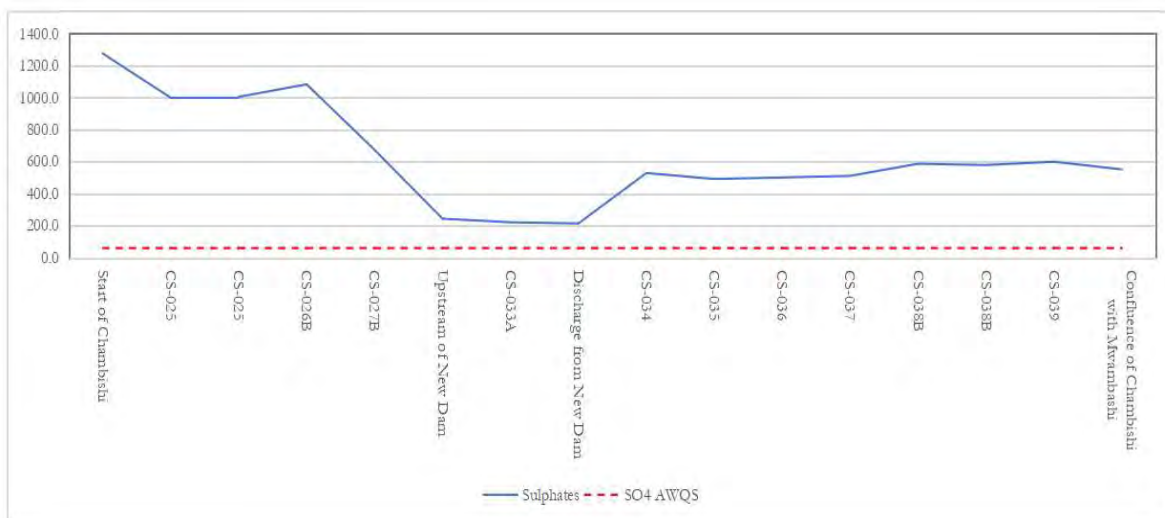
Figure 4-50: Concentration of sulphates in Chambishi Stream
