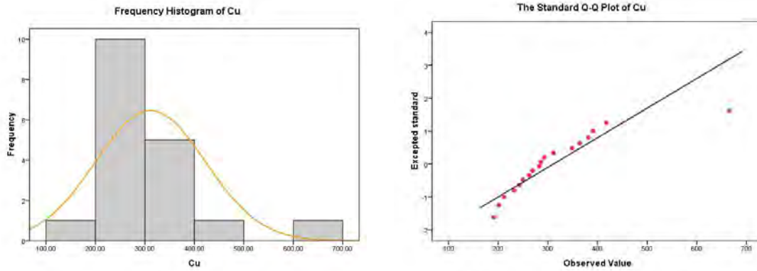
Figure 6-31: Frequency histogram and Q-Q diagram of Cu
