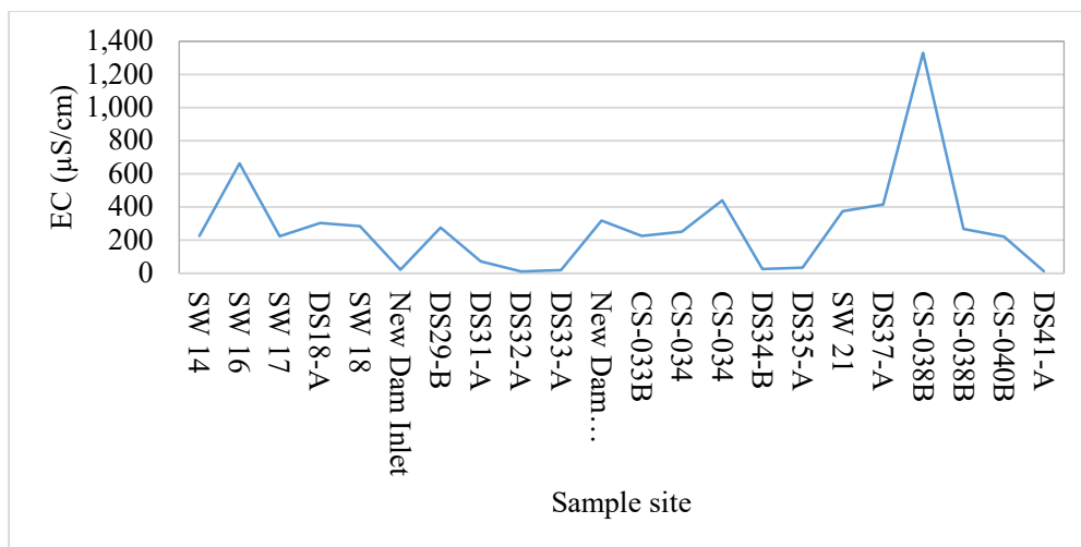
Figure 4-22: Graph showing EC in sediment
