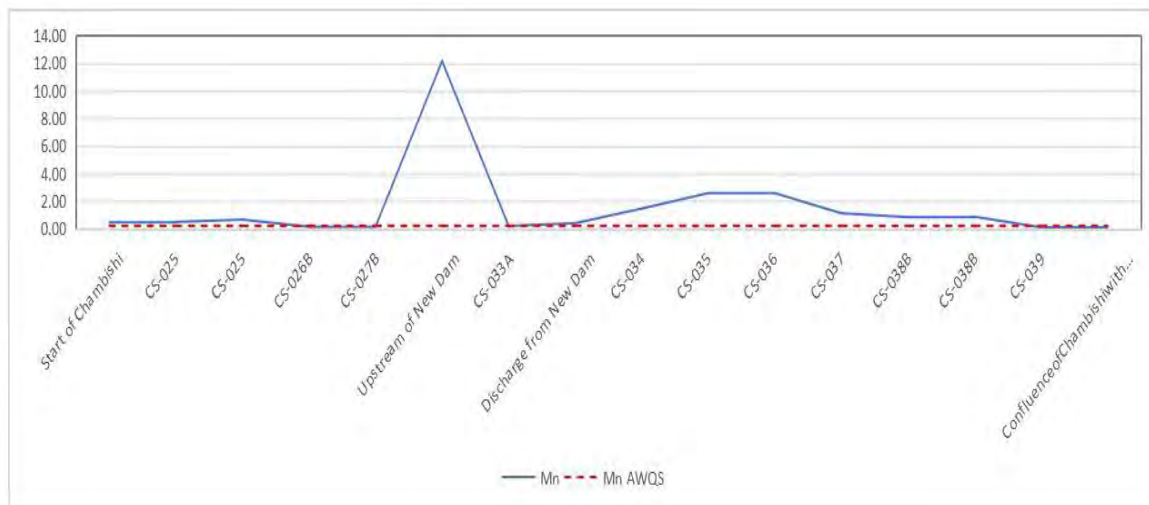
Figure 4-49: Concentration of manganese in Chambishi Stream
