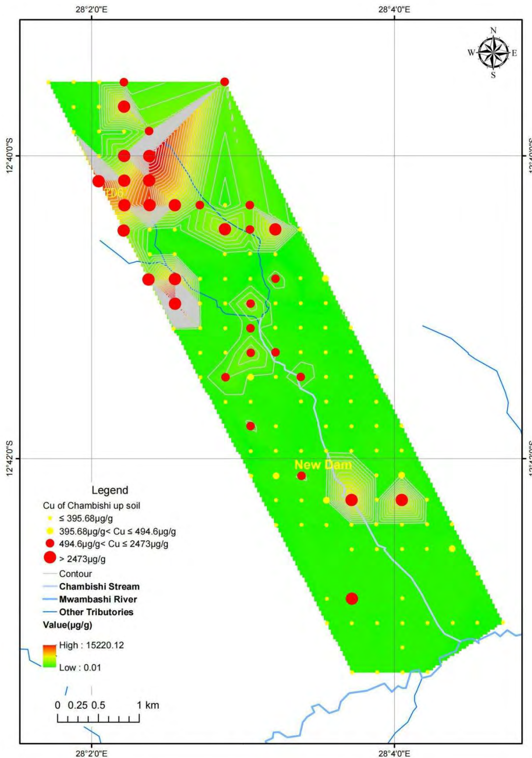
Figure 6-42: Distribution of Cu Exceeding Baseline Value
