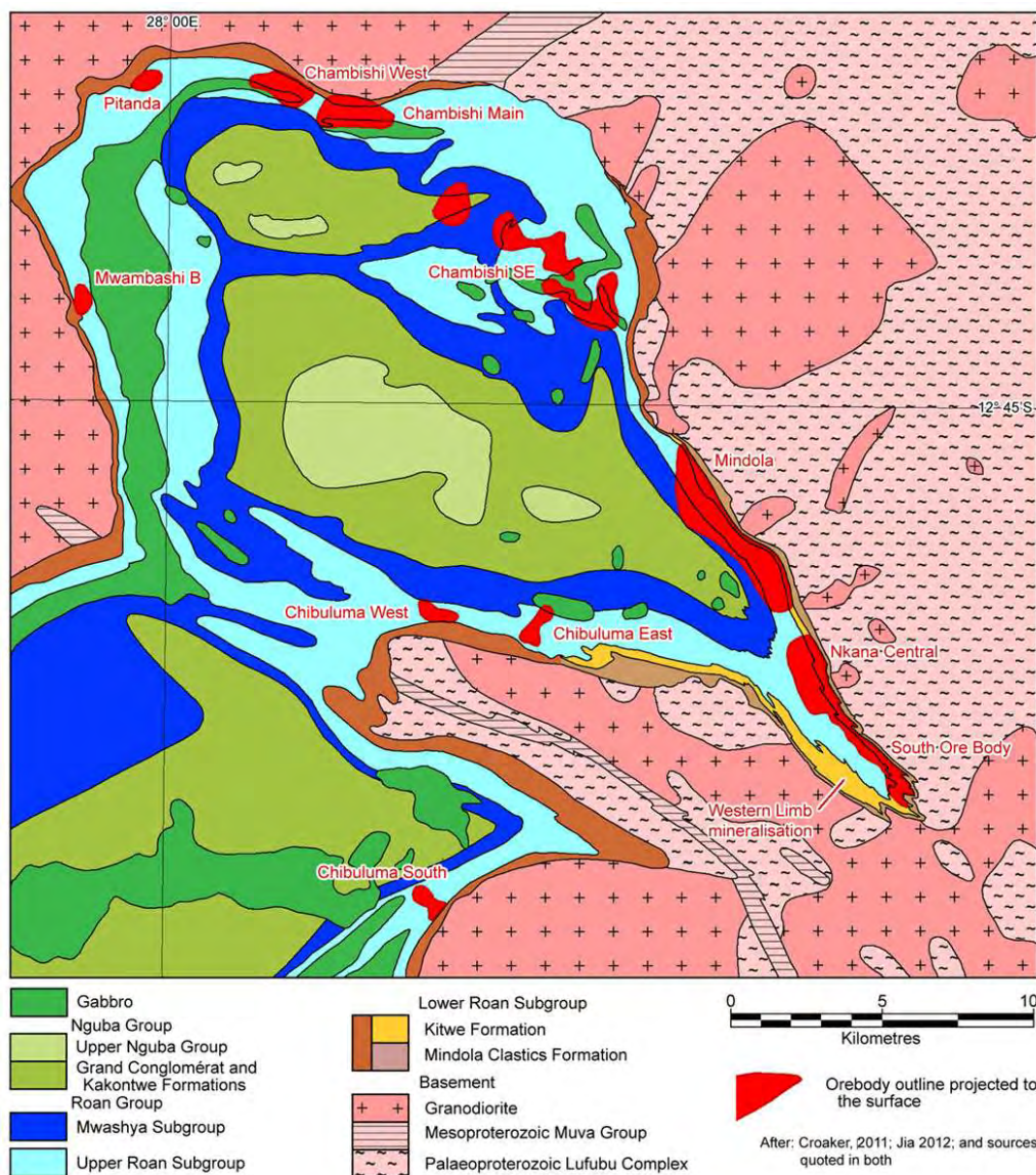
Figure 5-9: Geological setting of the Chambishi basin 11
