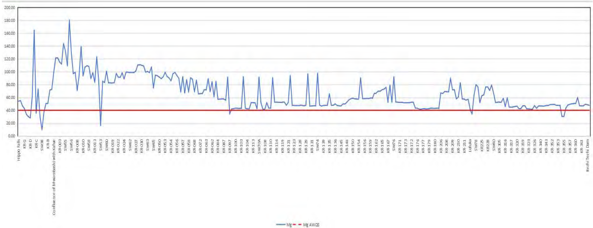
Figure 4-67: Concentration of magnesium in Kafue River
