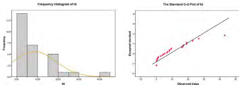
Figure 6-38: Frequency histogram and Q-Q diagram of Ni
