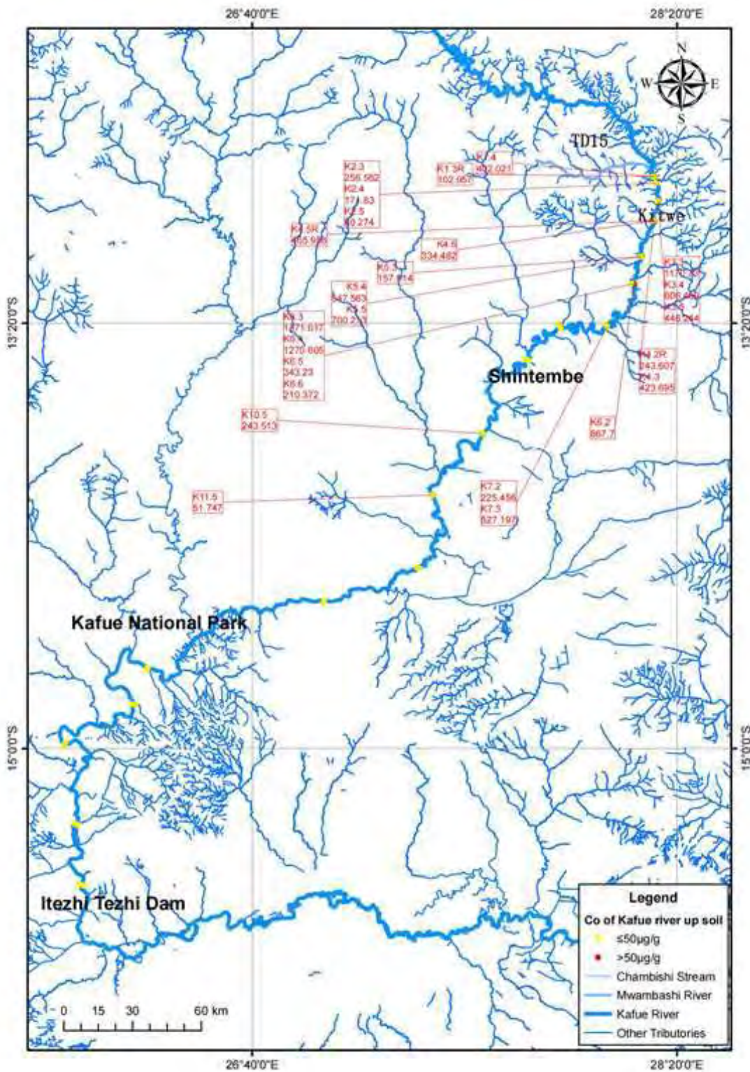
Figure 6-23: Distribution of Cobalt in Kafue River
