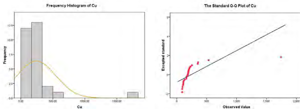
Figure 6-37: Frequency histogram and Q-Q diagram of Cu
