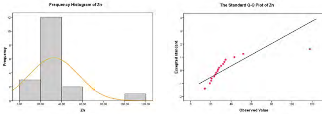
Figure 6-34: Frequency histogram and Q-Q diagram of Zn
