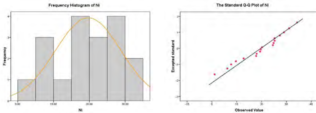
Figure 6-32: Frequency histogram and Q-Q diagram of Ni
