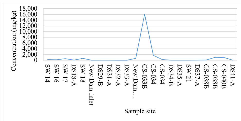
Figure 4-24 showing the concentration of Cobalt in sediment
