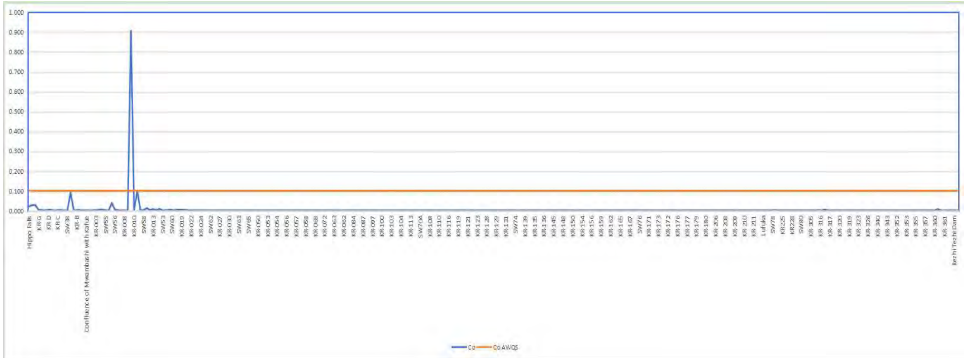
Figure 4-64: Concentration of cobalt in Kafue River
