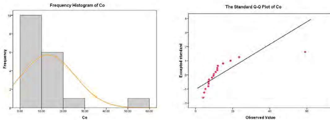
Figure 6-30: Frequency histogram and Q-Q diagram of Co
