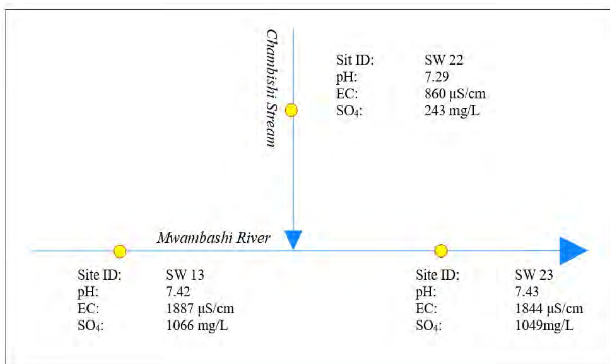
Figure 4-73: Schematic drawing illustrating the impact of Chambishi Stream on the water quality of Mwambashi River
