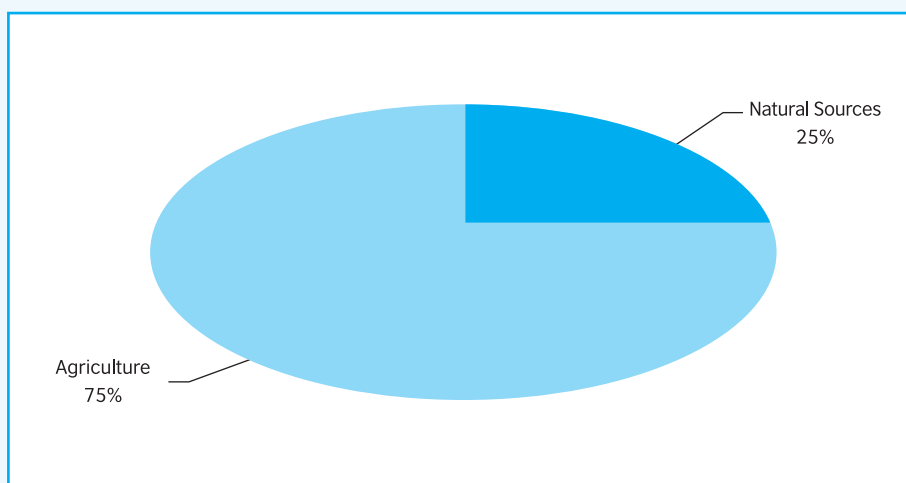
Figure 2.10: Percentage contribution by sector to total NH 3 emissions for Zambia
