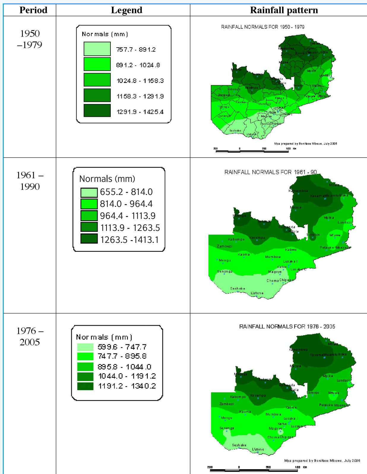
Figure 2.14: Rainfall Normals over periods 1950 – 1979, 1961 – 1990, 1976 – 2005
