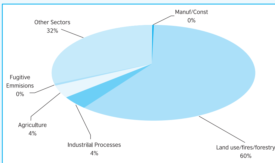
Figure 2.11: Percentage contributions by sector to total PM 10 emissions
