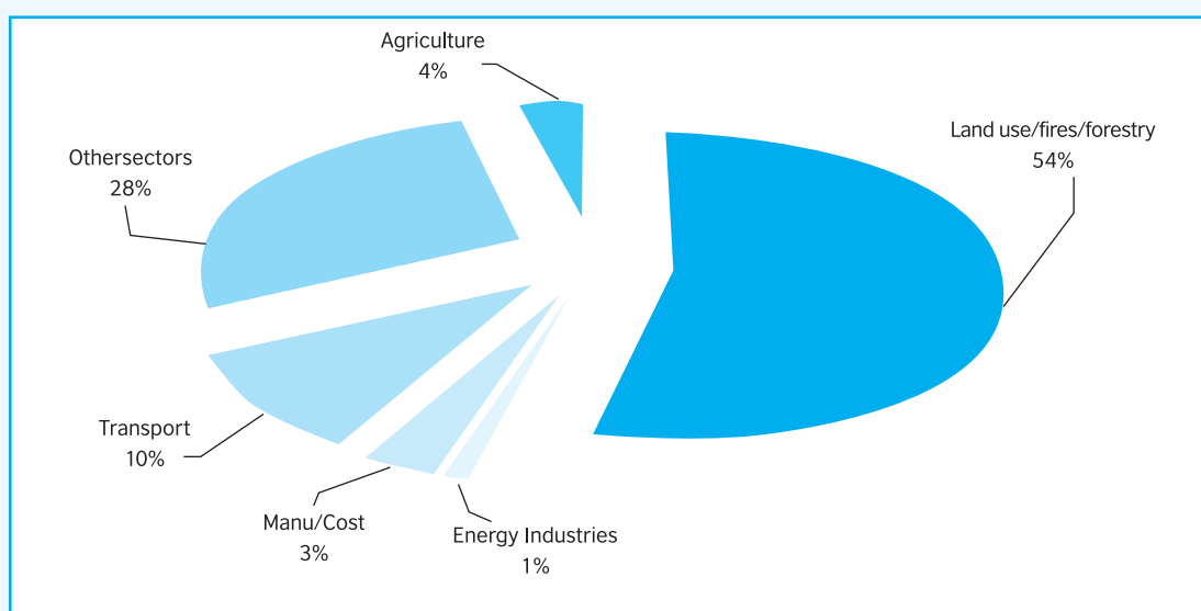
Figure 2.8: Percentage contribution by sector to total NO x emissions for Zambia
