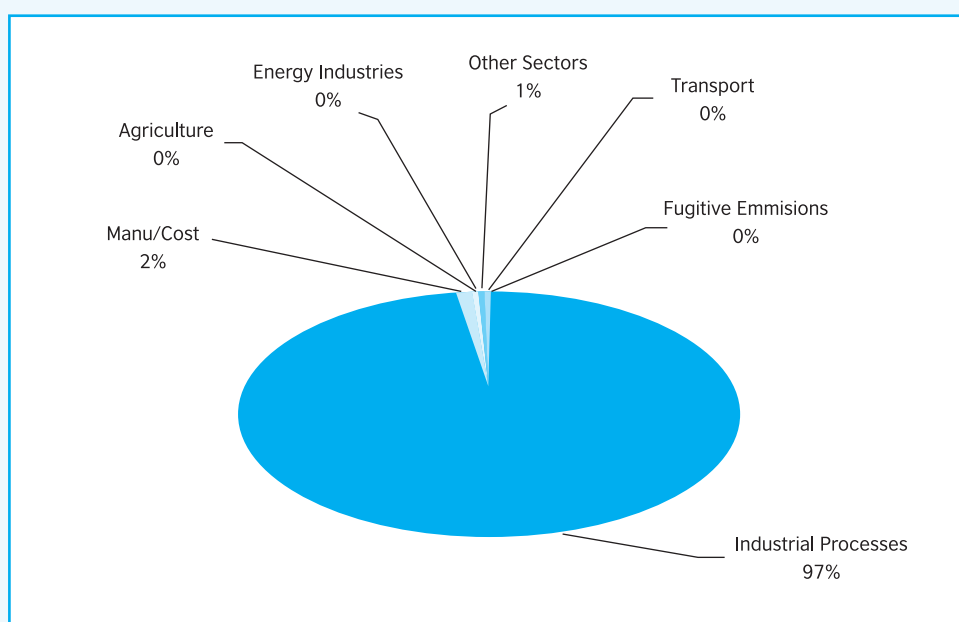
Figure 2.6: Percentage contribution by sector to total Sulphur dioxide (SO 2 ) Emissions.
