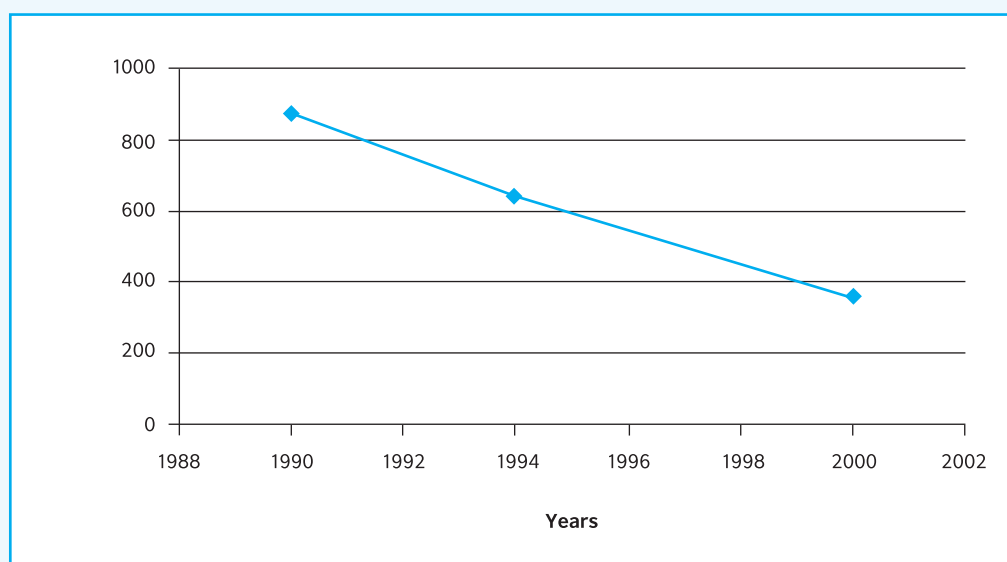
Figure 2.7: Trends in SO 2 emissions in Zambia (1990, 1994 and 2000)
