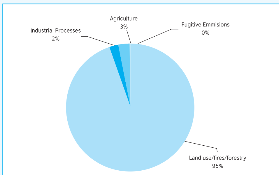
Figure 2.12: Percentage contribution by sector to total PM2.5 emissions in 2000
