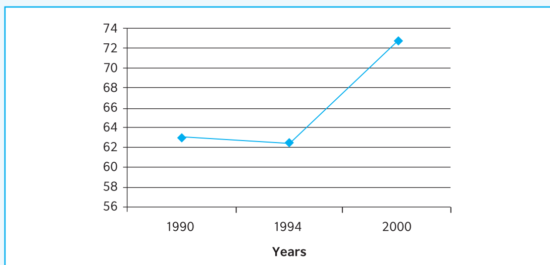
Figure 2.9: Trend of NO x emissions in Zambia using 1990, 1994 and 2000 data
