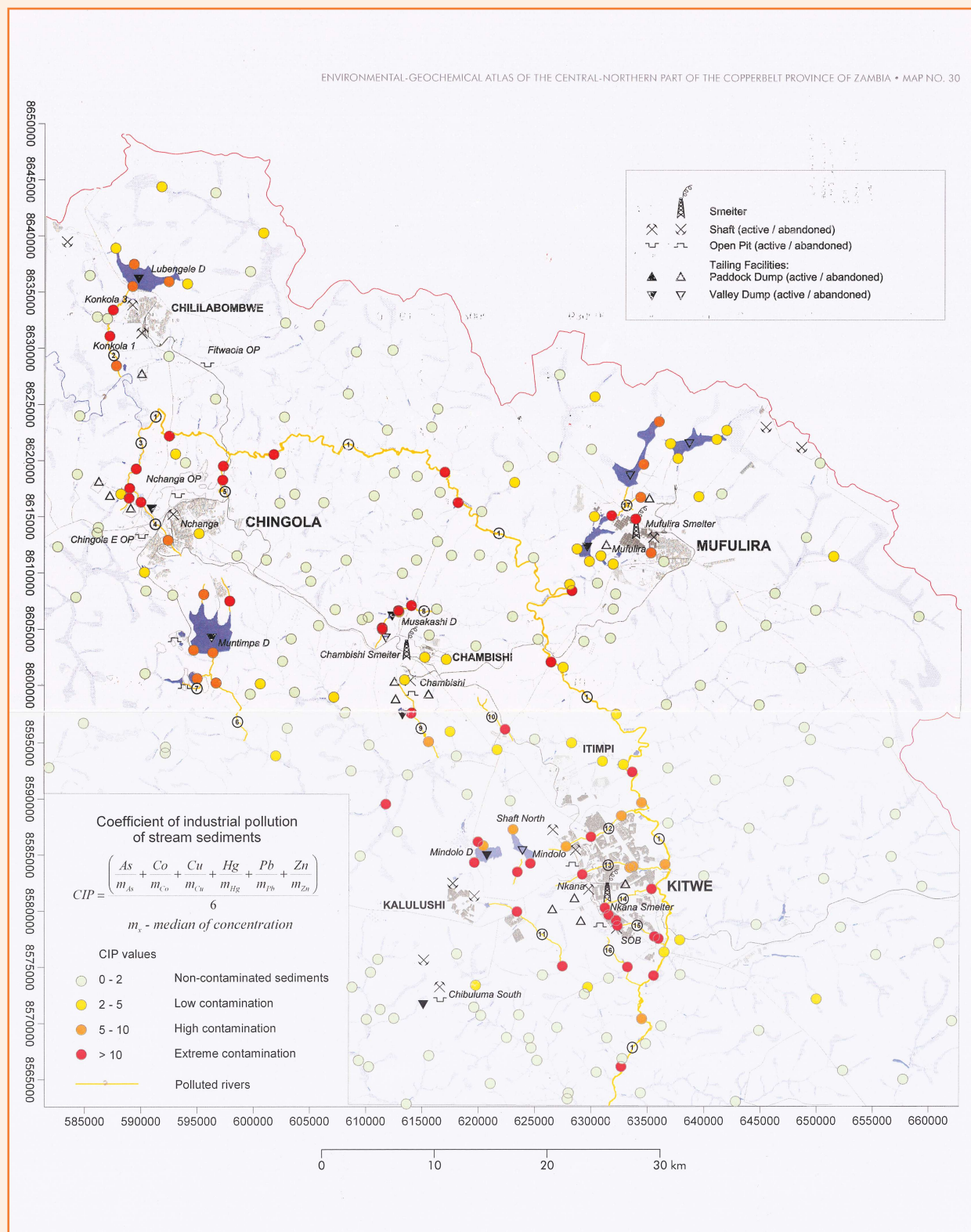
Figure 6.18: Concentration of Cu in stream sediments.
